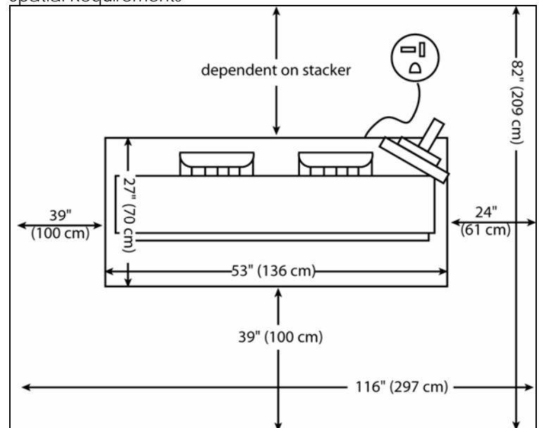
Top View, Not to Scale.
