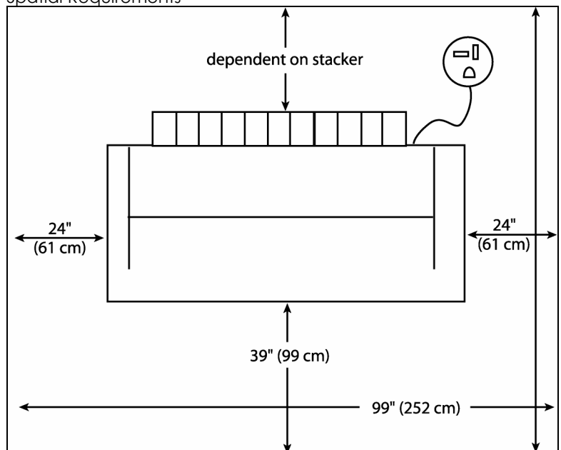
Top View, Not to Scale. Shown with standard print rack
